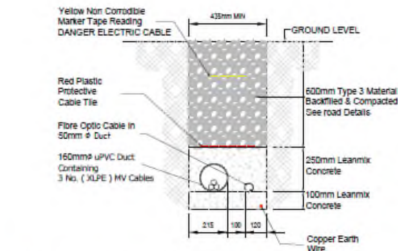
CABLE TRENCH IN SITE ROADWAY SINGLE CIRCUIT ( INTERNAL WIND FARM ) Scale 1:20
